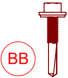
#12 x 1-1/4" SCREW Part#: 20201
