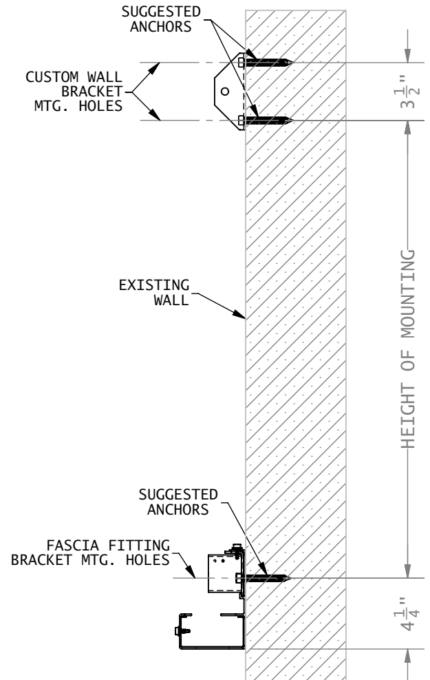
ASSEMBLED DETAIL VIEW
