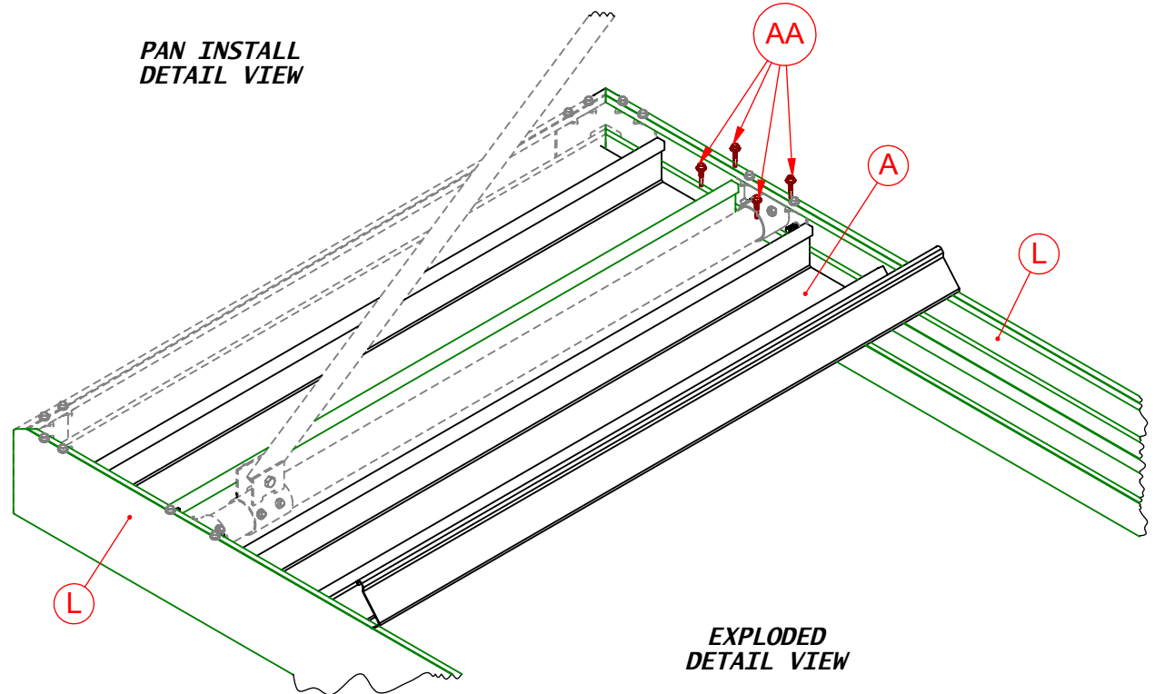
#8 x 3/4" SCREW Part# 20123
