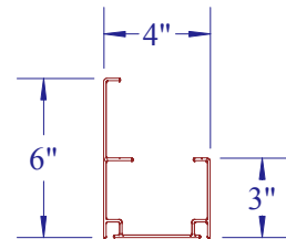
GUTTER PROFILE
