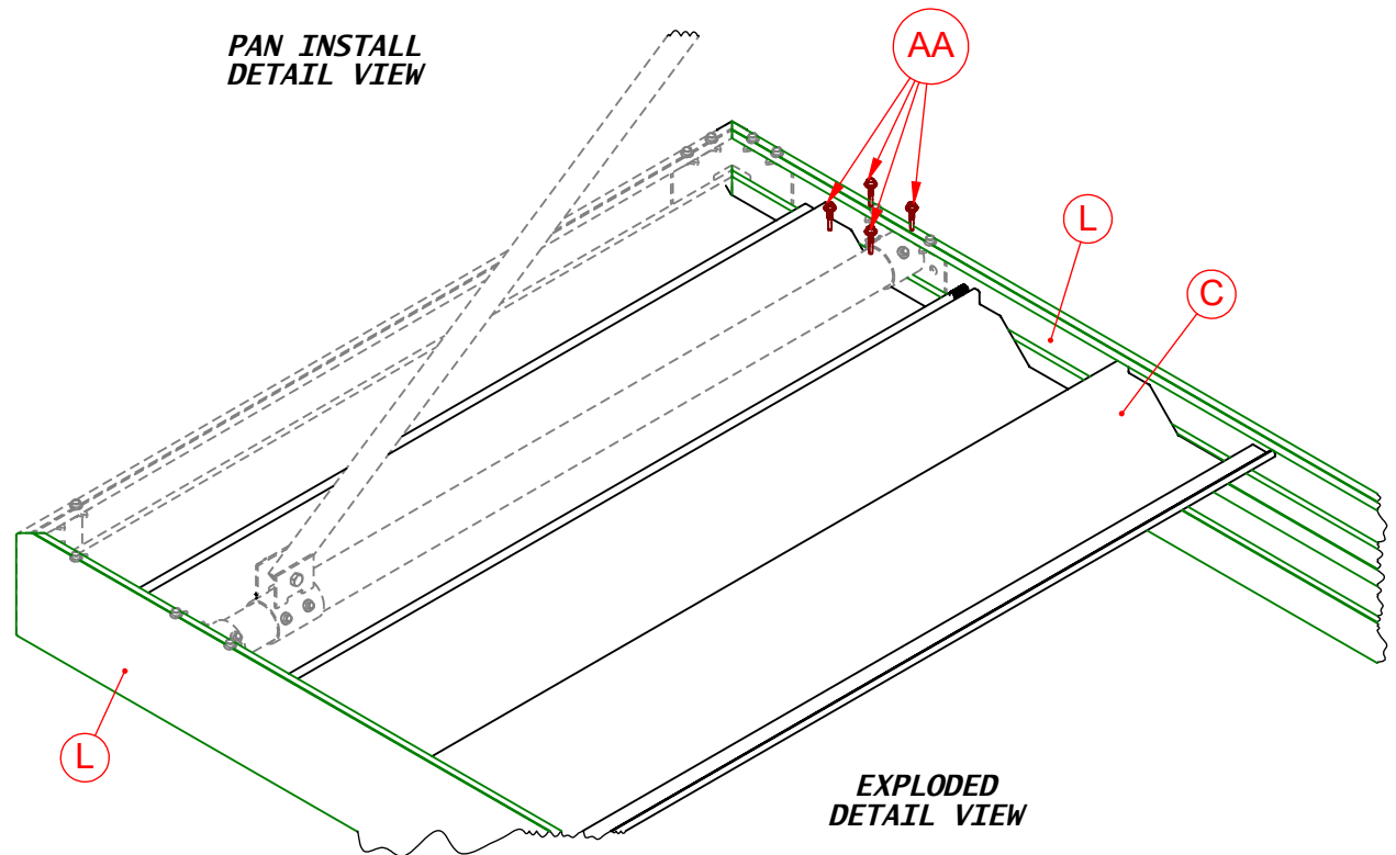
#8 x 3/4" SCREW Part# 20123
